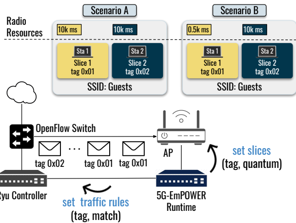
Fig. 3: Network deployment used for the demonstration.
