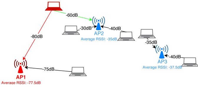
Fig. 1: Average RSSI indicator triggering a handover as condition (\text{Max}(\text{AvRSSI}) - \text{Min}(\text{AvRSSI})) > \text{Med}(\text{AvRSSI}) is met ( 77.5 - 35 > 37.5 ).
